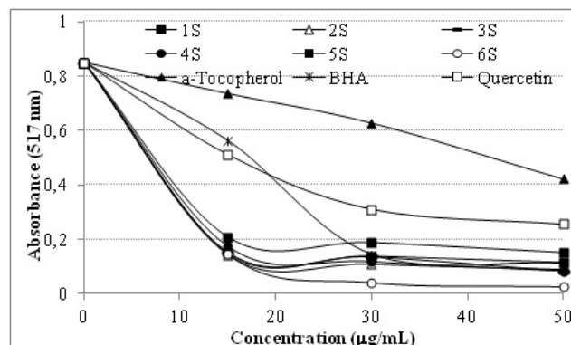
Figure 4. DPPH free radical scavenging activity of different concentrations (15, 30, 50 \mu\text{g}/\text{mL} ) of phenolic compounds (1-6) and standard antioxidant \alpha -tocopherol, BHA, quercetin.
