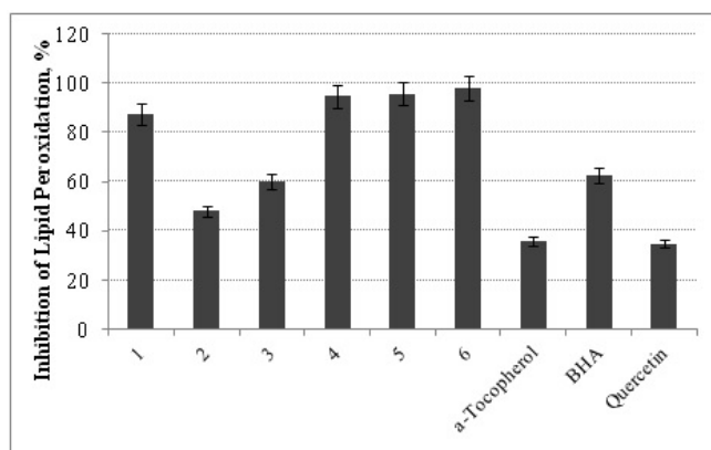
Figure 2. Comparison the percentages of inhibition of lipid peroxidation of phenolic compounds (1-6) in 30 \mu\text{g}/\text{mL} concentration with \alpha -tocopherol, BHA, and quercetin (30 \mu\text{g}/\text{mL} ) as standard antioxidant (BHA: butylated hydroxyanisole).
