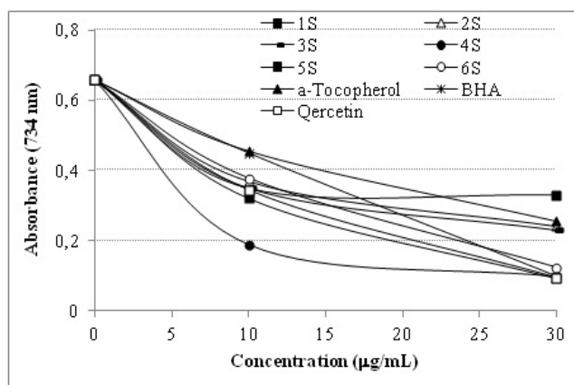
Figure 5. ABTS •+ radical scavenging activity of different concentrations (10, 30 µg/ml) of phenolic compounds (1–6) and standart antioxidant α-Tocopherol, BHA, Quercetin.
