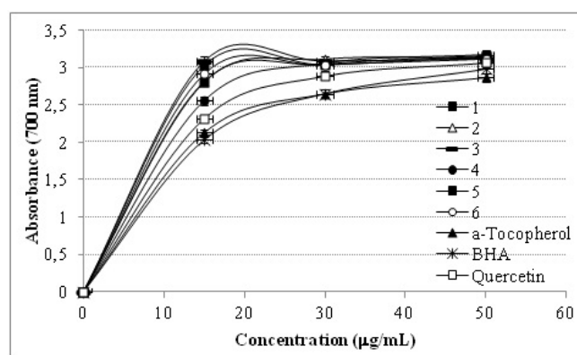
Figure 3. Total reduction potential of (1-6) phenolic compounds of different concentrations (15, 30, 50 \mu\text{g}/\text{mL} ) and standard antioxidant \alpha -tocopherol, BHA and quercetin.
